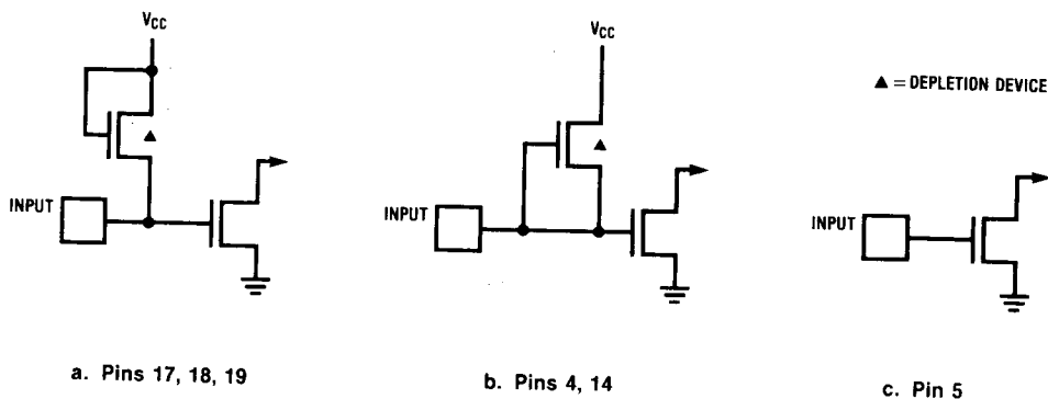
Figure 4. Input Configurations
