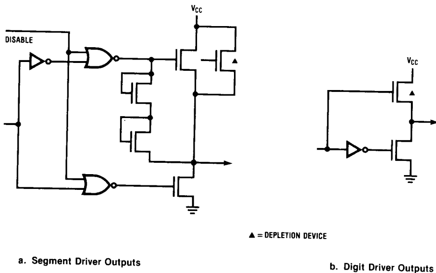
Figure 5. Output Configurations
