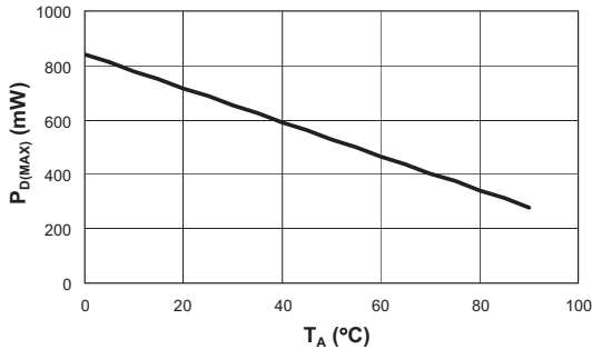
Figure 3: Maximum Power Dissipation.
