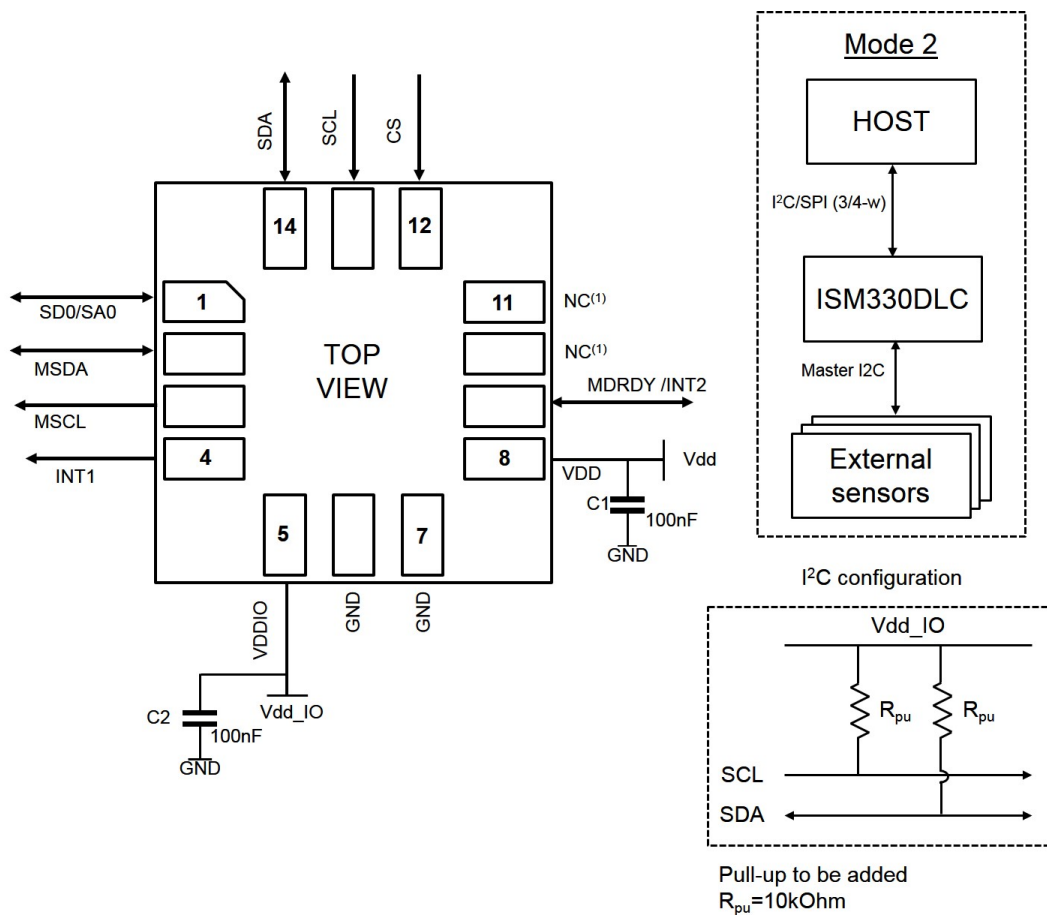
Figure 18. ISM330DLC electrical connections in Mode 2
