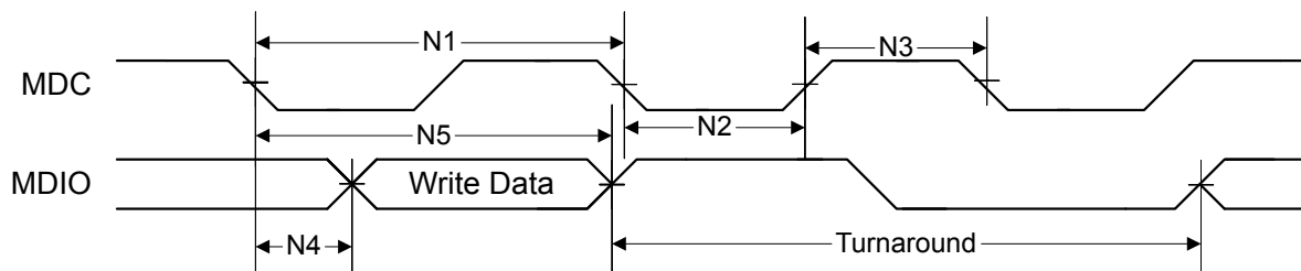
Figure 27-26. Station Management Write Timing
