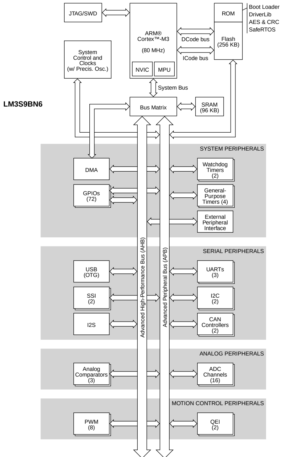
Figure 1-1. Stellaris® LM3S9BN6 Microcontroller High-Level Block Diagram
