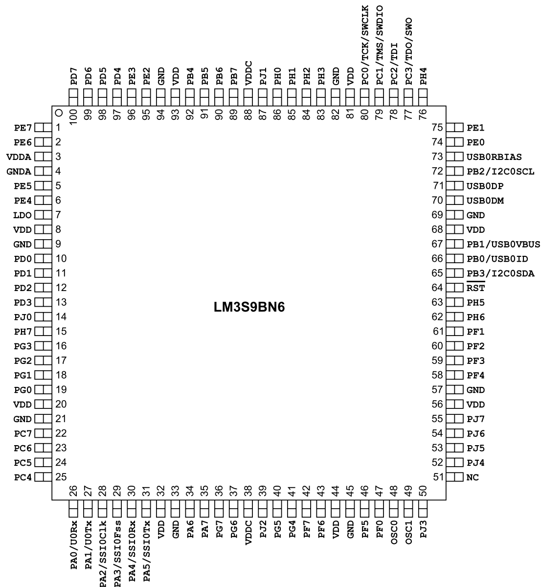
Figure 24-1. 100-Pin LQFP Package Pin Diagram
