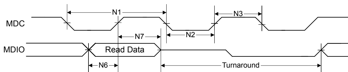
Figure 27-27. Station Management Read Timing
