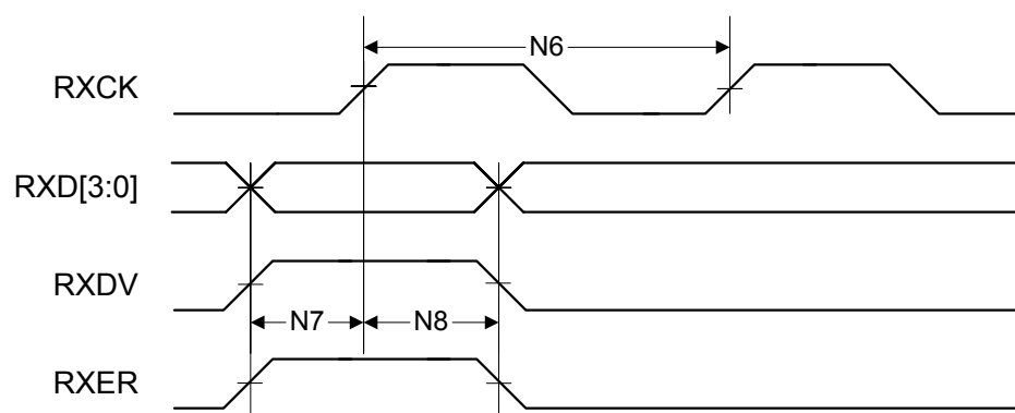
Figure 27-28. MII Receive Timing
