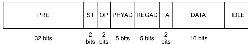
Figure 19-4. Management Frame Format
