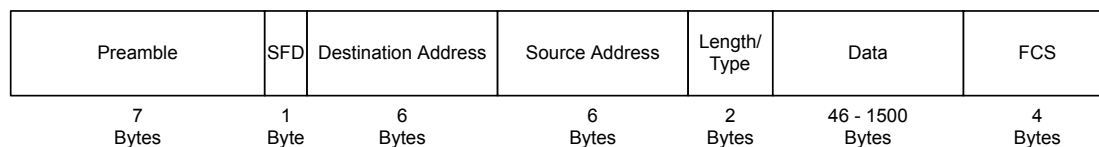
Figure 19-3. Ethernet Frame
