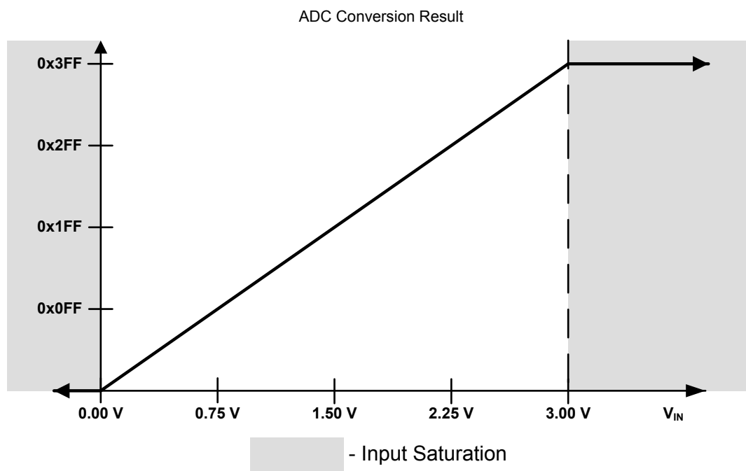
Figure 13-6. Internal Voltage Conversion Result
