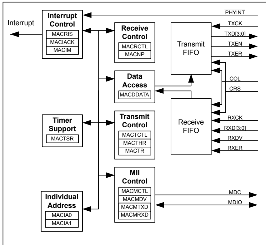
Figure 19-2. Ethernet MAC Block Diagram
