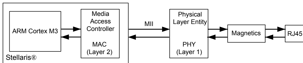
Figure 19-1. Ethernet Controller
