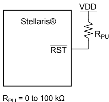
Figure 6-1. Basic \overline{RST} Configuration
