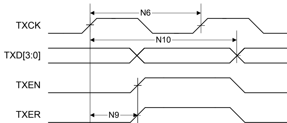
Figure 27-29. MII Transmit Timing
