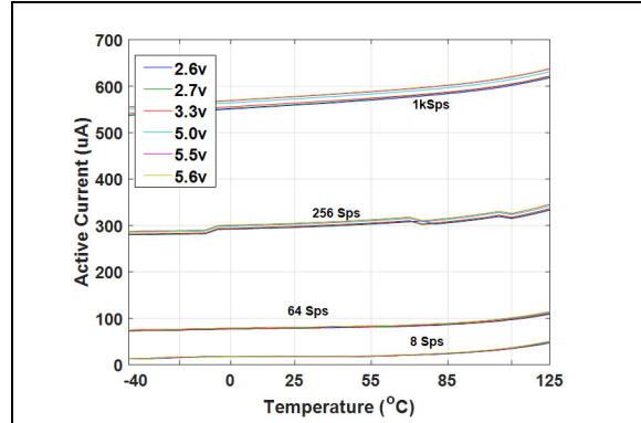
FIGURE 2-22: I_{DD} vs. Temperature, V_{DD} , and Sample Rate.
