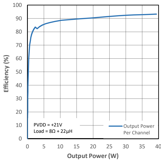
Figure 15-12 PMP4 Efficiency (VDD+PVDD) vs Output Power
