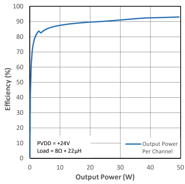
Figure 13-12 PMP4 Efficiency (VDD+PVDD) vs Output Power
