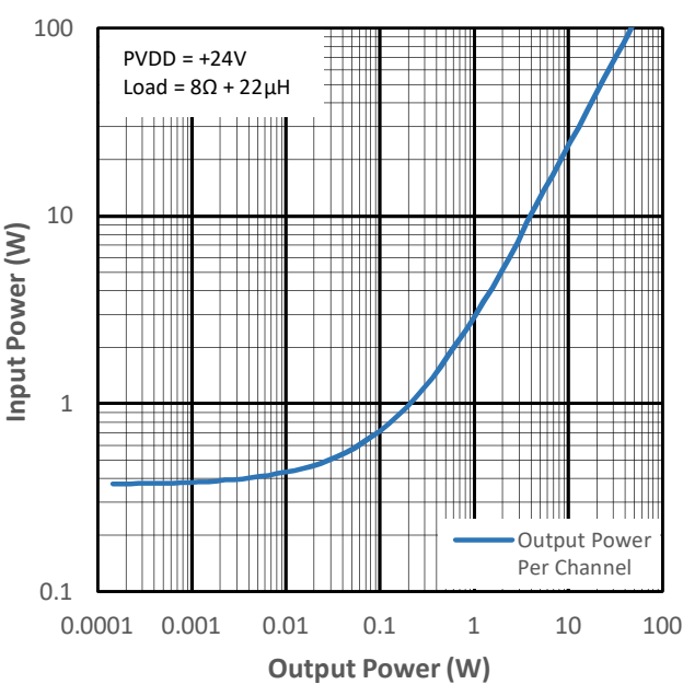
Figure 13-14 Input Power vs Output Power for PMP1
