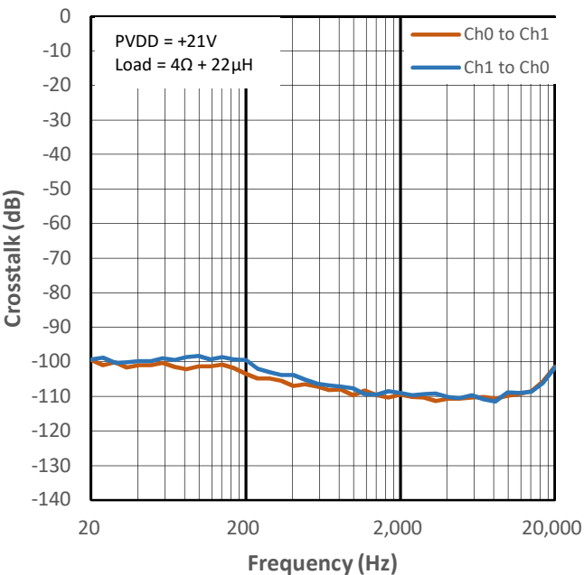
Figure 14-28 Crosstalk vs Frequency for PMP4
