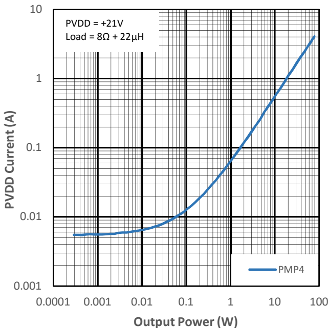
Figure 15-20 PVDD Current vs Output Power for PMP4
