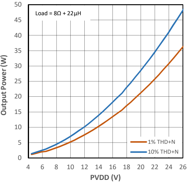
Figure 11-21 Output Power vs PVDD for PMP0
