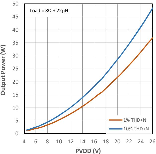
Figure 11-24 Output Power vs PVDD for PMP4
