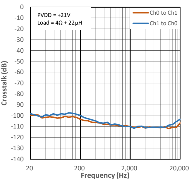
Figure 14-26 Crosstalk vs Frequency for PMP1
