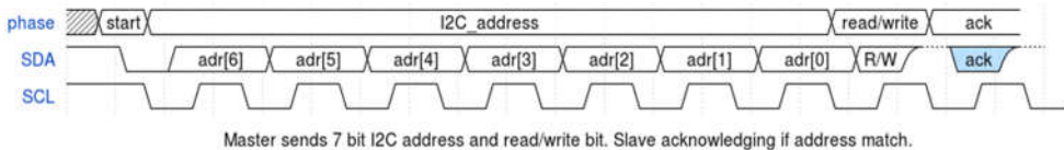
Figure 8-8. I2C init addressing sequence.
