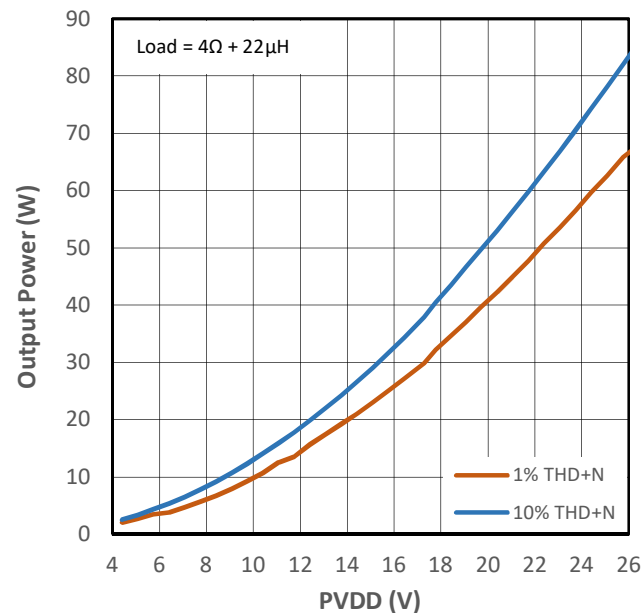
Figure 10-22 Output Power vs PVDD for PMP1
