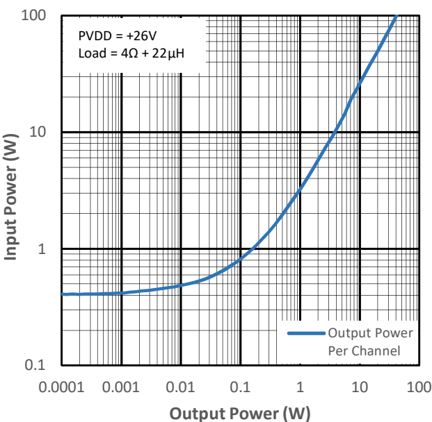
Figure 10-14 Input Power vs Output Power for PMP1
