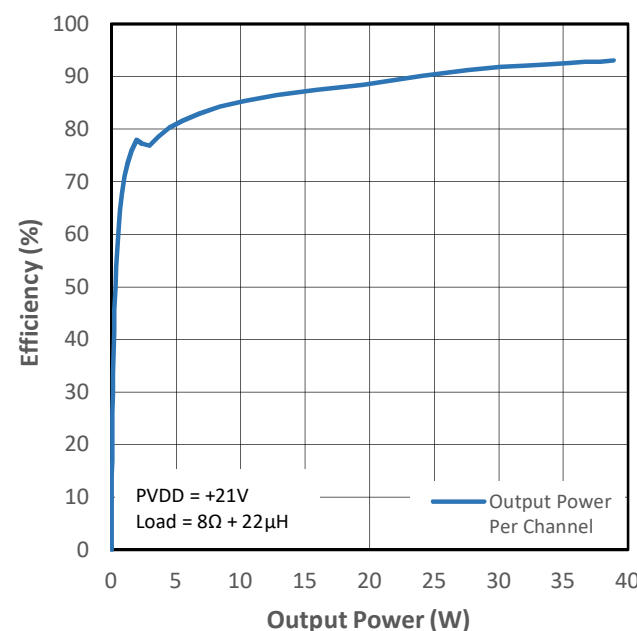
Figure 15-10 PMP1 Efficiency (VDD+PVDD) vs Output Power
