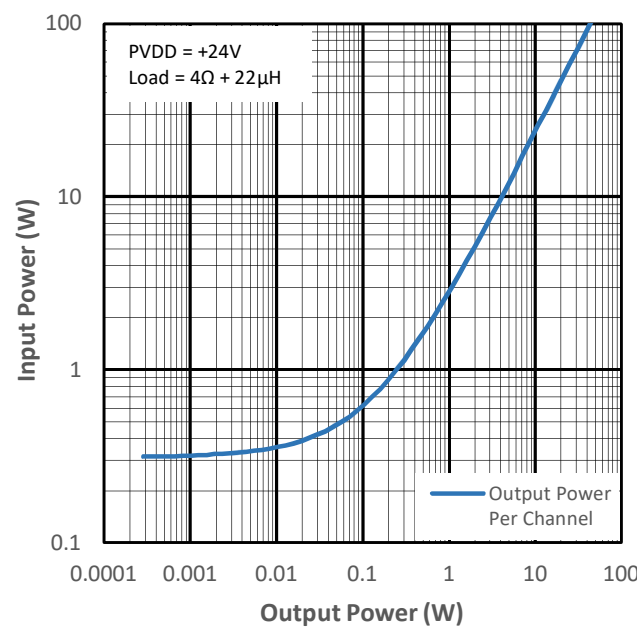
Figure 12-16 Input Power vs Output Power for PMP4
