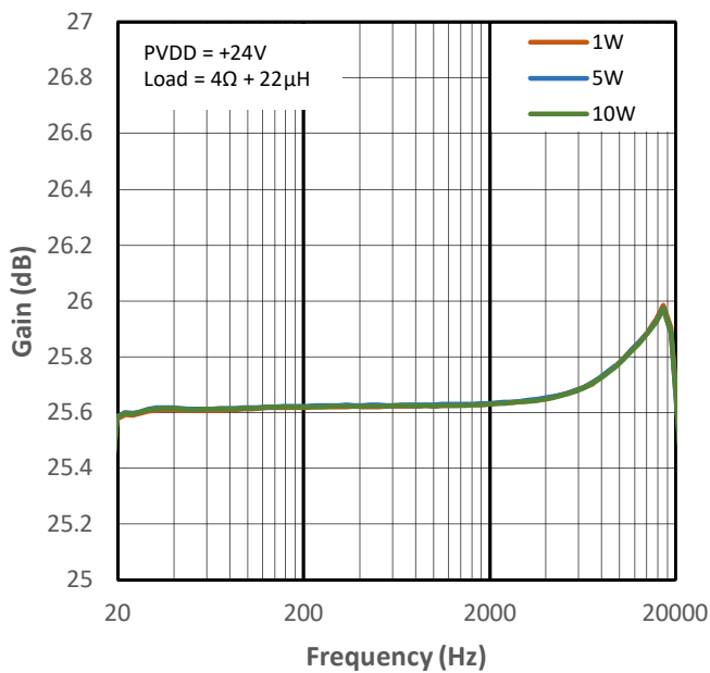
Figure 12-24 Gain vs Frequency for PMP4
