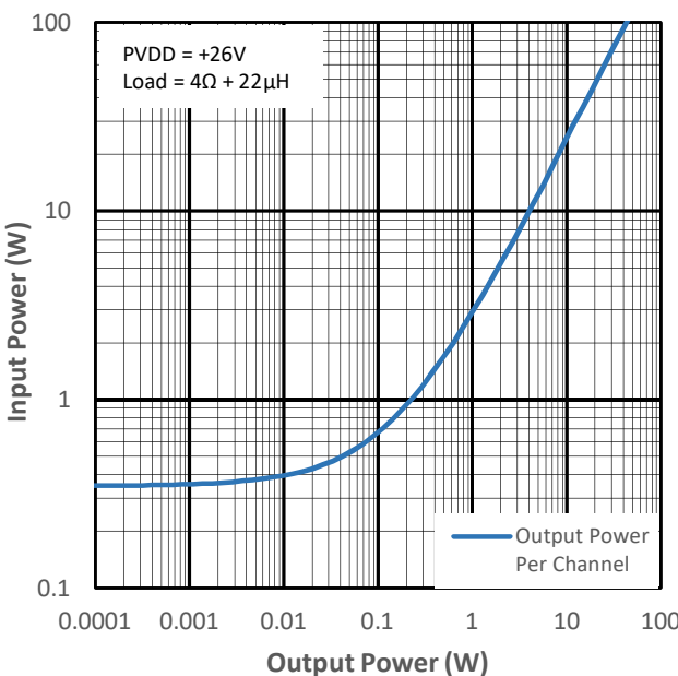
Figure 10-16 Input Power vs Output Power for PMP4
