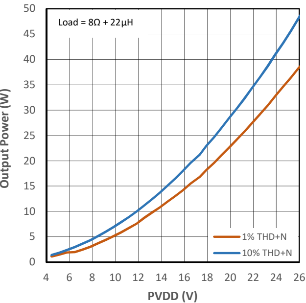
Figure 11-23 Output Power vs PVDD for PMP2
