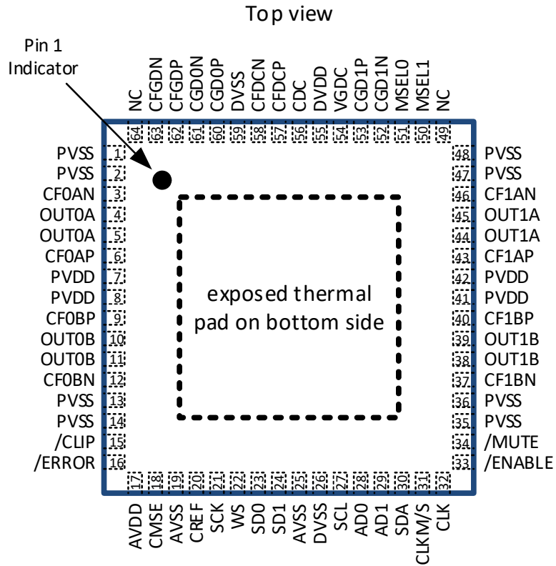
Figure 4-1 Pinout MA12070PQFN
