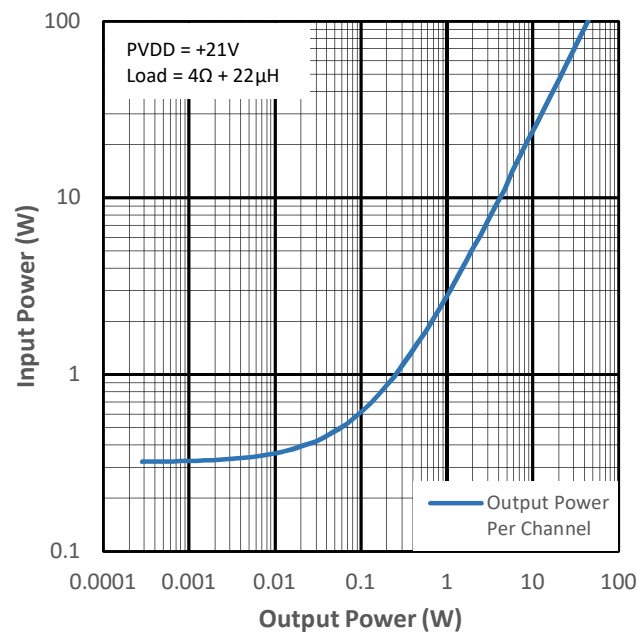
Figure 14-16 Input Power vs Output Power for PMP4
