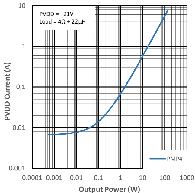
Figure 14-20 PVDD Current vs Output Power for PMP4
