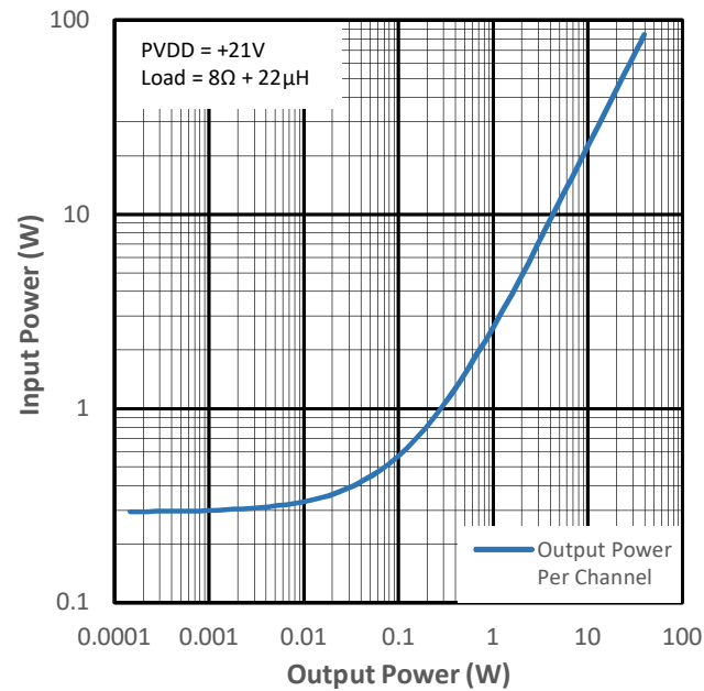
Figure 15-16 Input Power vs Output Power for PMP4
