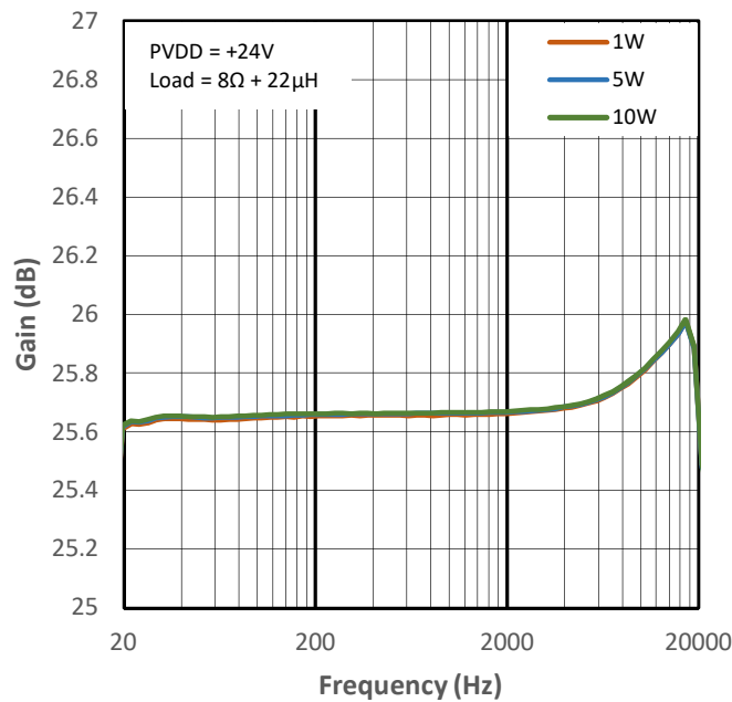
Figure 13-24 Gain vs Frequency for PMP4
