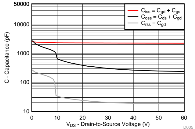
Figure 5. Capacitance
