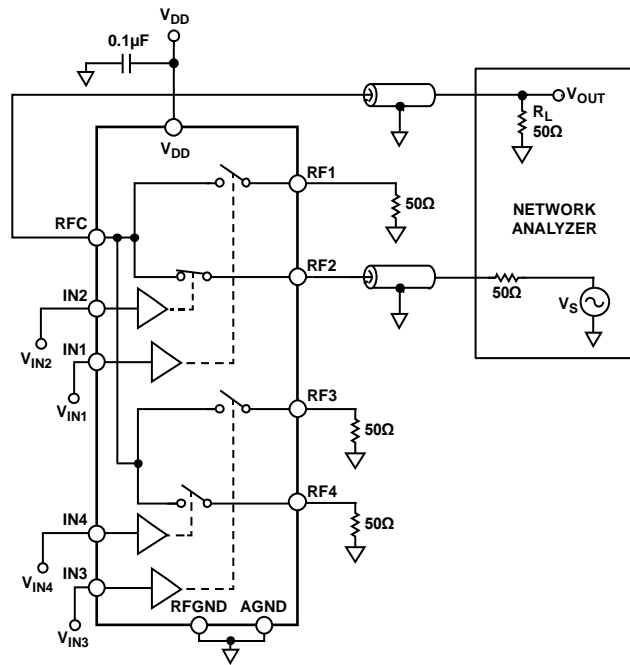
Figure 23. Insertion Loss/Return Loss
