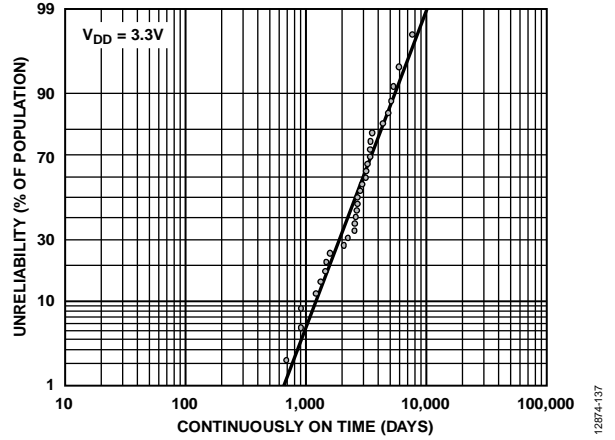
Figure 43. Continuously on Lifetime, V DD = 3.3 V, 50°C, Sample Size 31 Parts
