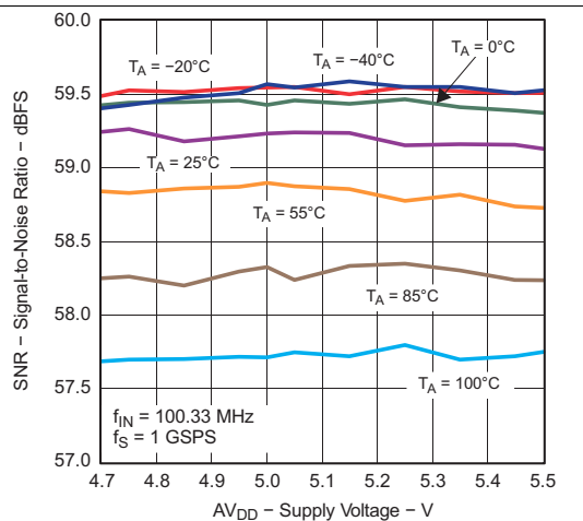
Figure 17. SNR vs AVDD5 Across Temperature
