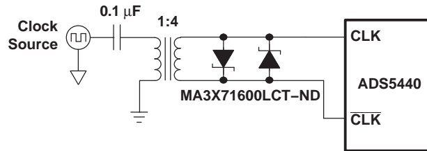
Figure 40. Differential Clock
