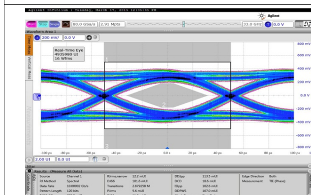
Figure 78. Eye at 10-Gbps Bit Rate with Default Output Swing
