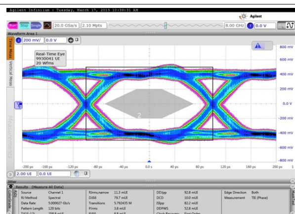
Figure 77. Eye at 5-Gbps Bit Rate with Increased Output Swing
