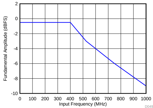
Figure 51. Maximum-Supported Amplitude vs Input Frequency
