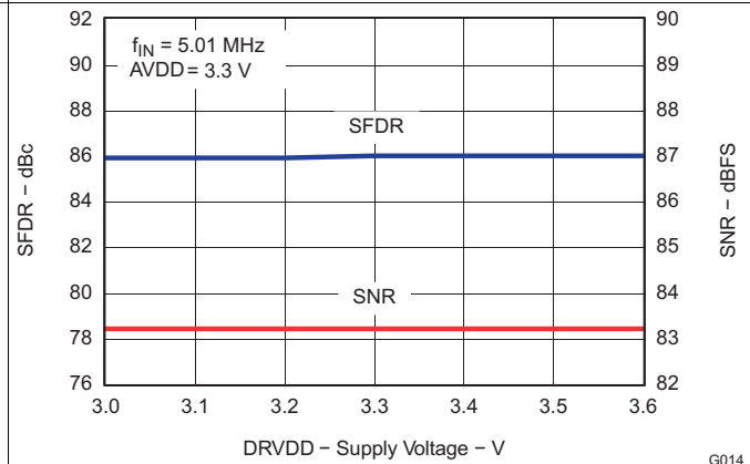
Figure 15. Performance vs DRVDD Supply
