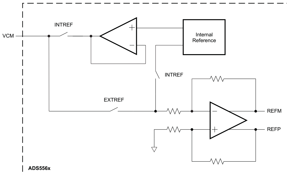
Figure 56. Reference Section
