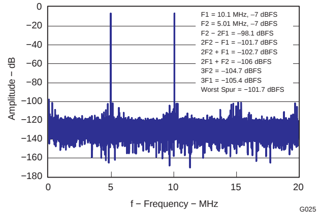
Figure 25. Intermodulation Distortion
