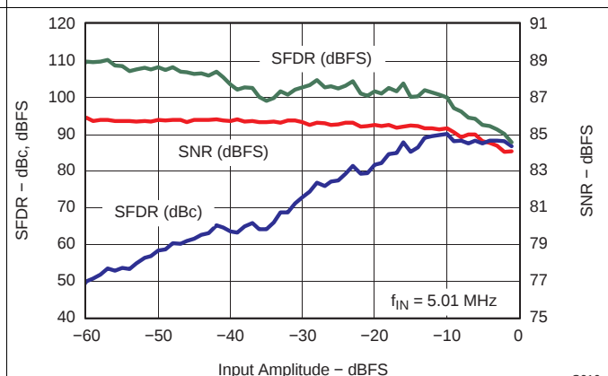
Figure 17. Performance vs Input Amplitude, 0-dB Gain
