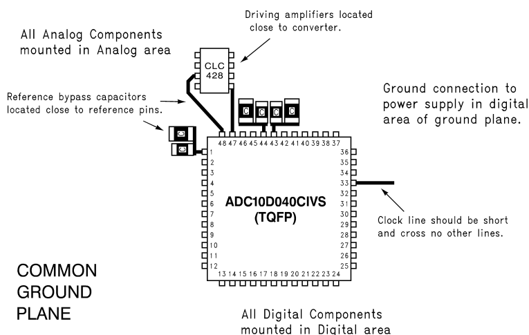
Figure 38. An Acceptable Layout Pattern
