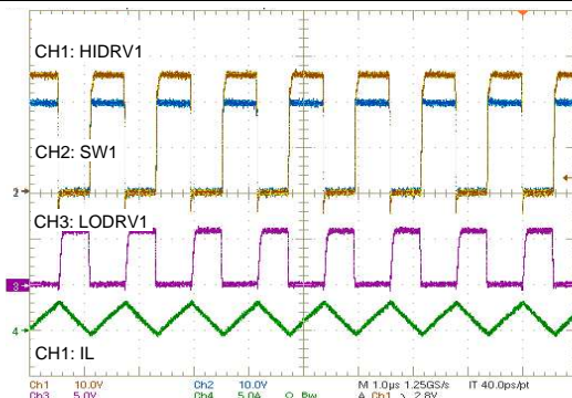
Figure 45. System Regulation
