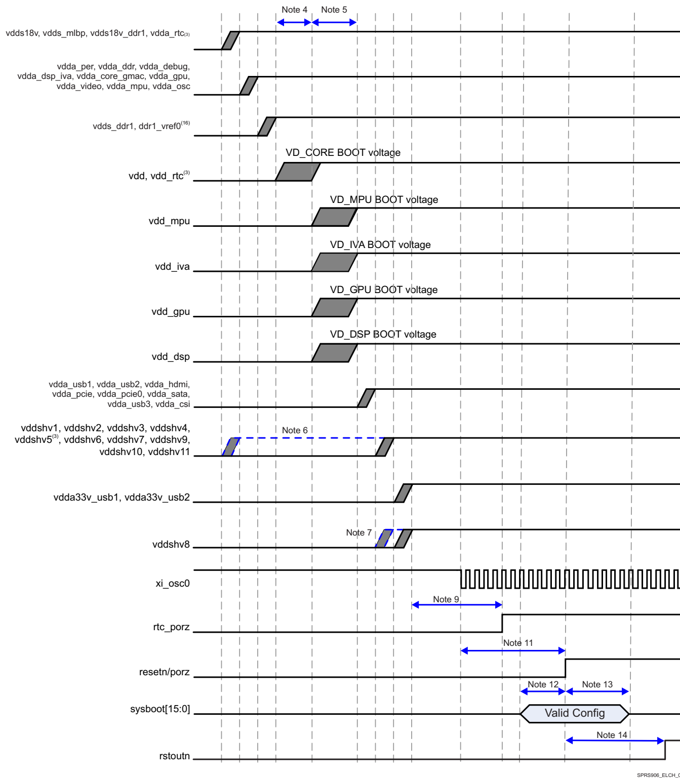
Figure 5-2. Power-Up Sequencing
