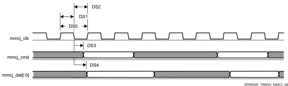
Figure 7-82. MMC/SD/SDIOj in - Default Speed - Transmitter Mode
