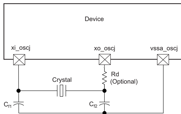
Figure 8-33. Grounding Scheme for High-Frequency Clock
