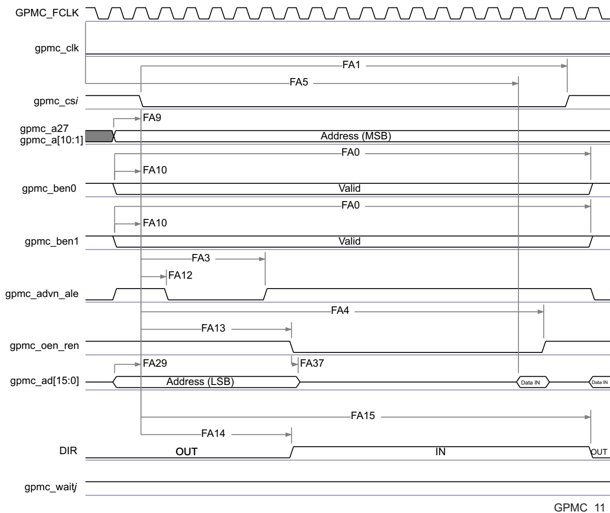
Figure 7-17. GPMC / Multiplexed NOR Flash - Asynchronous Read - Single Word Timing (1)(2)(3)
