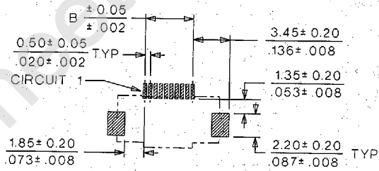
PCB LAYOUT: SOLDER SIDE
