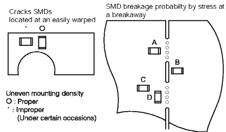
Fig.3 Component Layout
