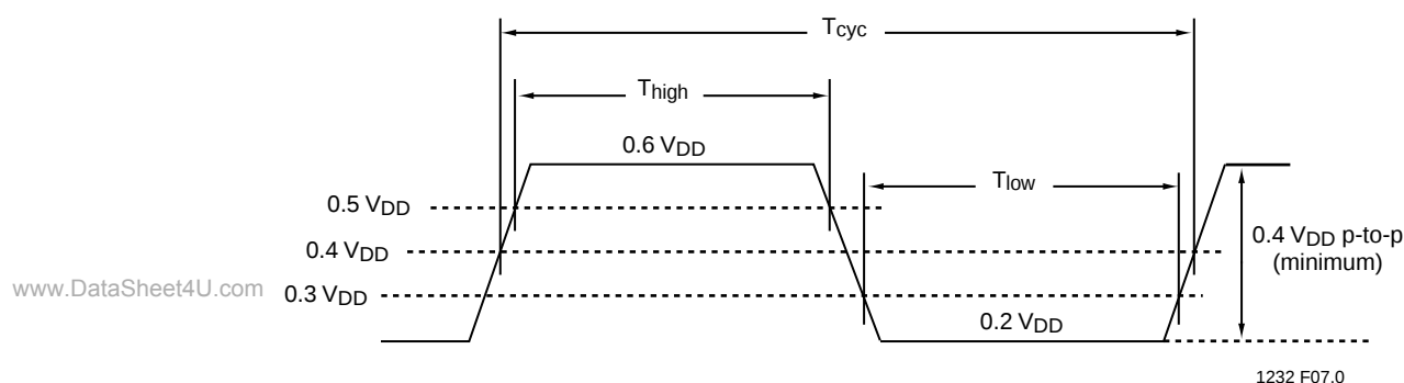
FIGURE 8: LCLK WAVEFORM (LPC MODE)
