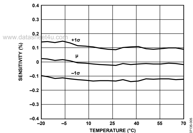
Figure 6. Gyroscope Sensitivity vs. Temperature
