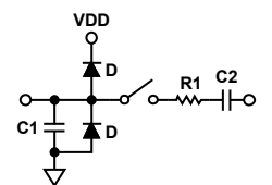
Figure 26. Equivalent Analog Input Circuit Conversion Phase: Switch Open Track Phase: Switch Closed
