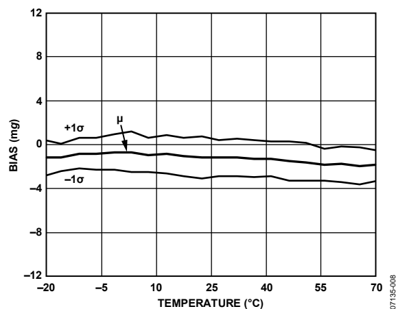
Figure 9. Accelerometer Bias vs. Temperature
