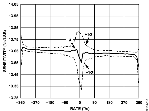
Figure 11. Gyroscope Linearity
