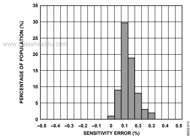
Figure 17. Accelerometer Sensitivity Error Distribution, +25°C
