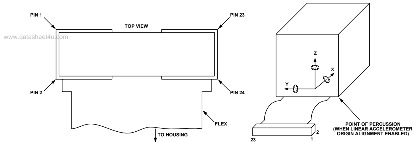
Figure 4. Pin Configuration, Connector Top View
