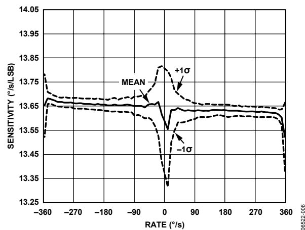
Figure 20. Gyroscope Linearity
