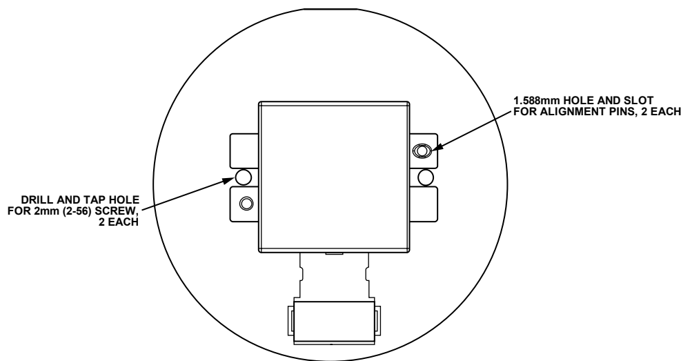
Figure 33. Mechanical Attachment
