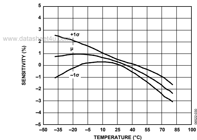
Figure 5. ADIS16350 Gyroscope Sensitivity vs. Temperature
