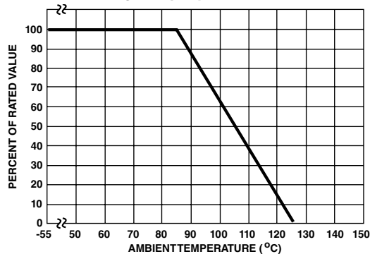
1A - Power Derating for Epoxy Coated
