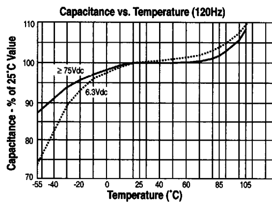
Type 350 Capacitance vs Temperature
