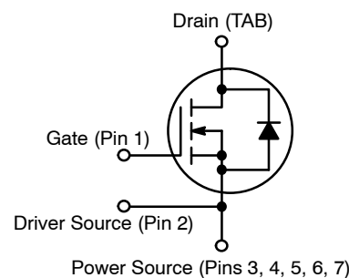
N-CHANNEL MOSFET
