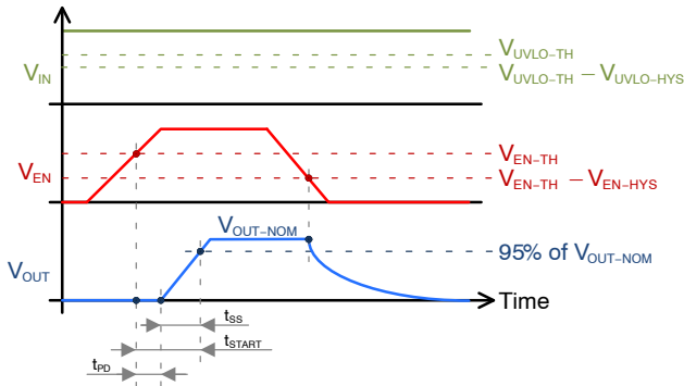
Figure 104. EN Pin Initiated Startup/Shutdown
