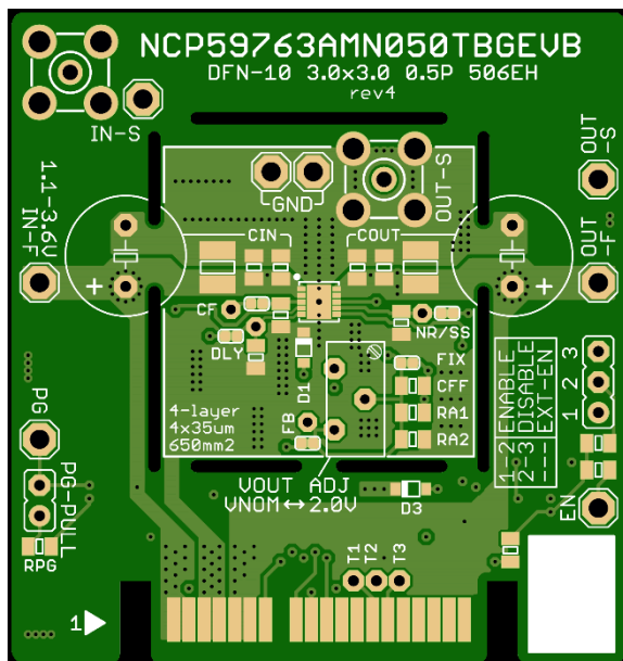
Figure 115. NCP59763AMN050TBGEVB Board
