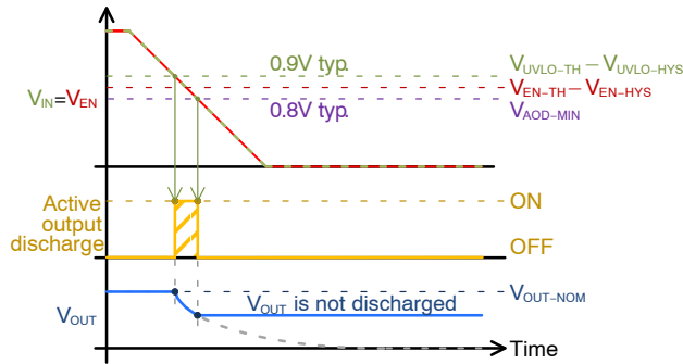
Figure 111. Active Output Discharge Activated by Falling V_{IN}
