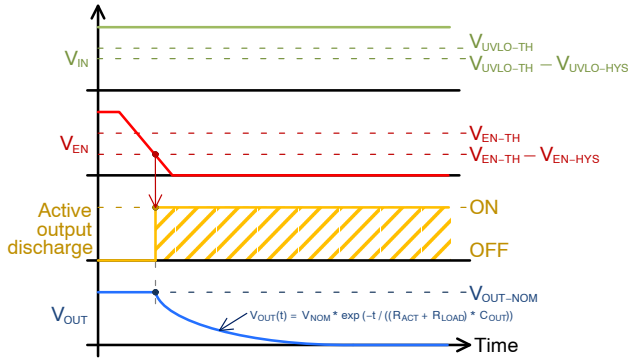
Figure 110. Active Output Discharge Activated by EN Pin
