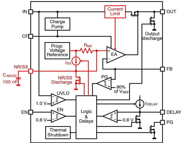
Figure 108. Internal Block Diagram (Startup Circuit Highlighted)
