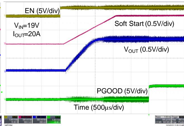
Figure 17. Startup Waveforms with 15 A Load Current
