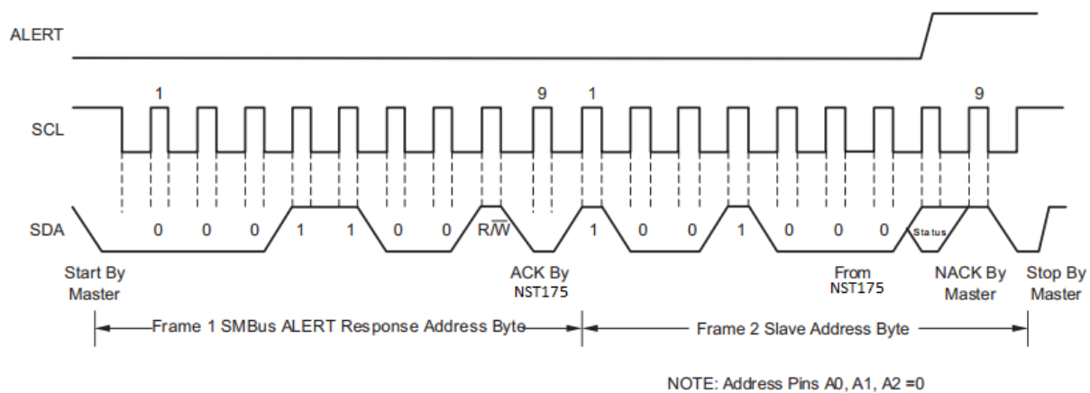
Figure 4.6. Timing Diagram for SMBus ALERT
