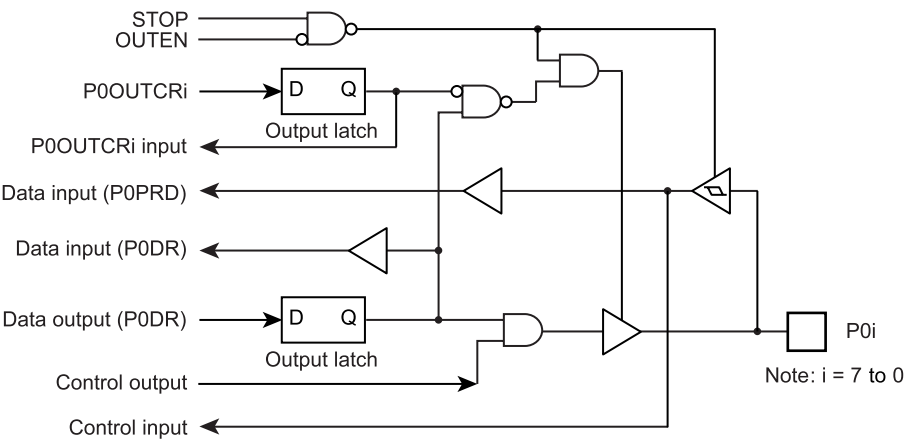
Figure 5-2 P0 Port
