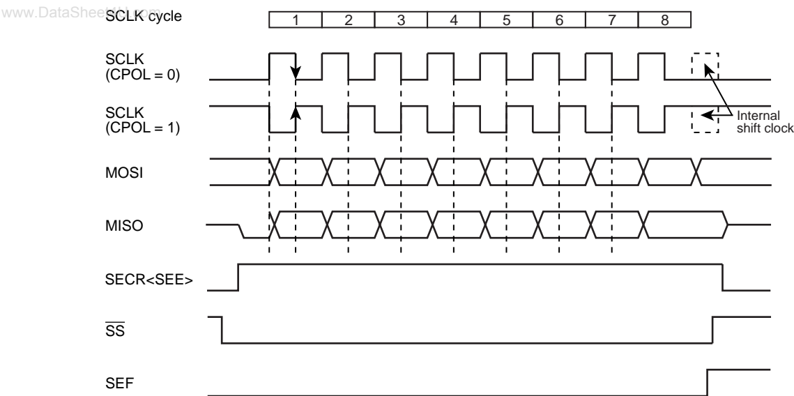
Figure 11-3 Transfer Format where CPHA = 1
