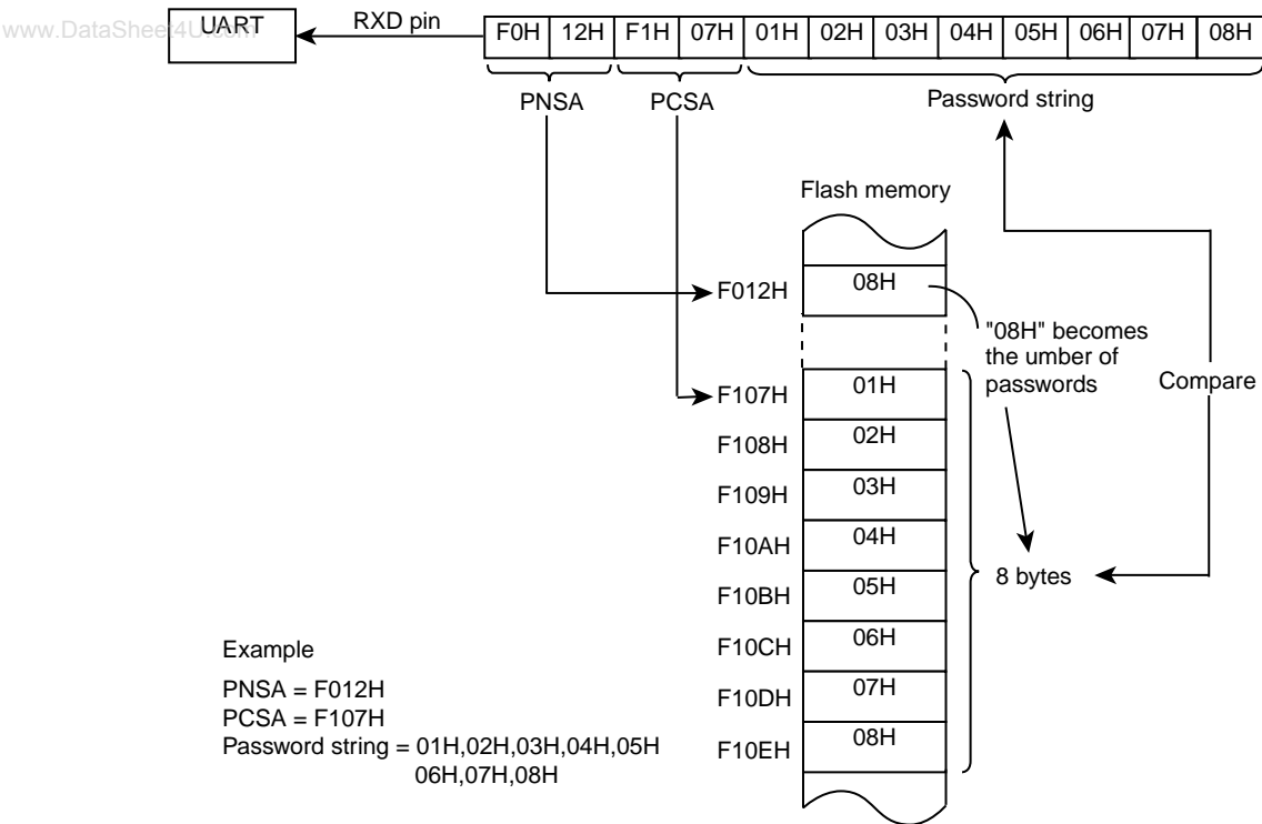
Figure 15-5 Password Comparison
