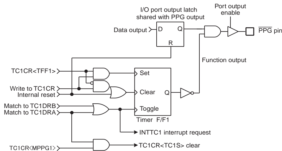
Figure 8-7 PPG Output
