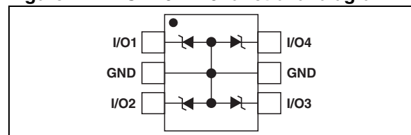
Figure 1. ESDA6V1P6 functional diagram
