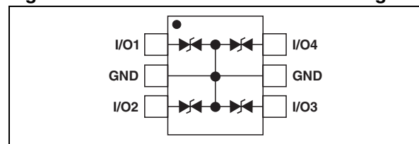
Figure 3. ESDA14V2BP6 functional diagram
