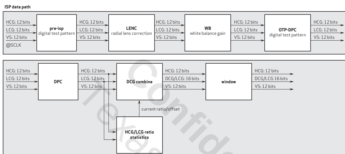
figure 4-1 image processor block diagram
