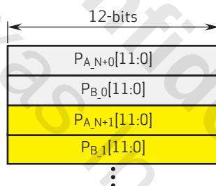
figure 5-24 12b RAW (HCG or LCG) + 12b VS diagram
