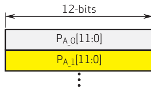
figure 5-23 12 bits linear mode diagram
