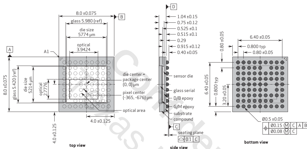
figure 9-1 package specifications
