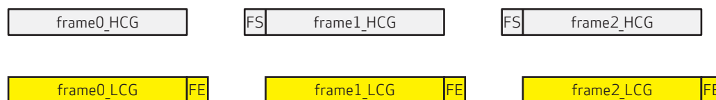
figure 5-7 non-staggered HDR without MIPI virtual channel overview diagram
