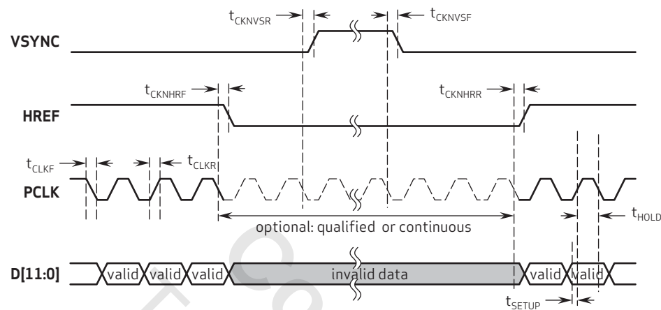
figure 5-20 DVP diagram
