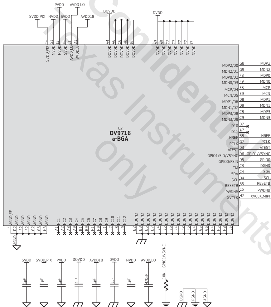
figure 1-4 OV9716 MIPI reference schematic
