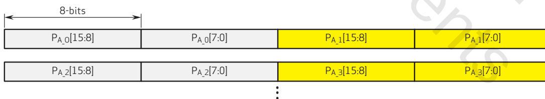
figure 5-16 16b DCG single HDR diagram
