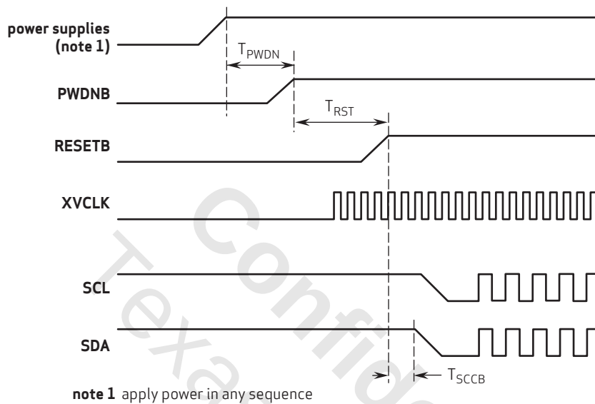
figure 1-6 power on timing diagram
