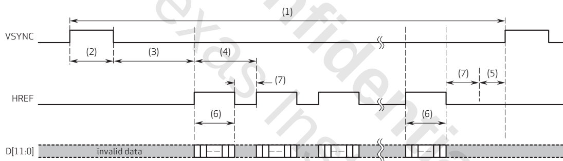
figure 5-21 DVP timing diagram
