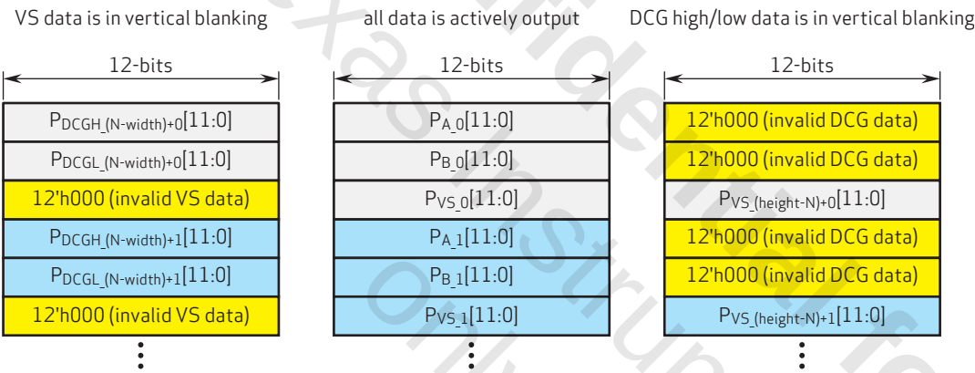
figure 5-22 staggered HDR with DVP diagram
