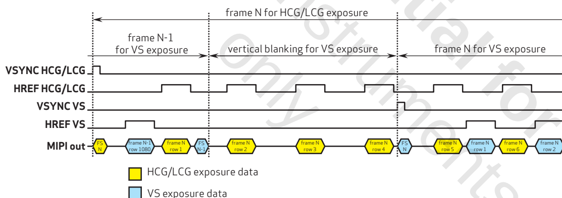
figure 5-6 staggered HDR with MIPI virtual channel detail diagram
