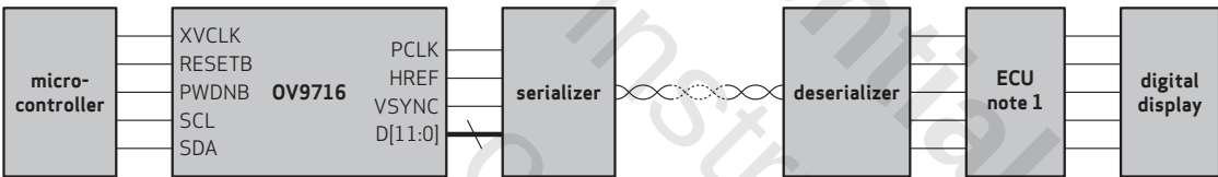
figure 1-1 standalone camera block diagram for automotive applications
