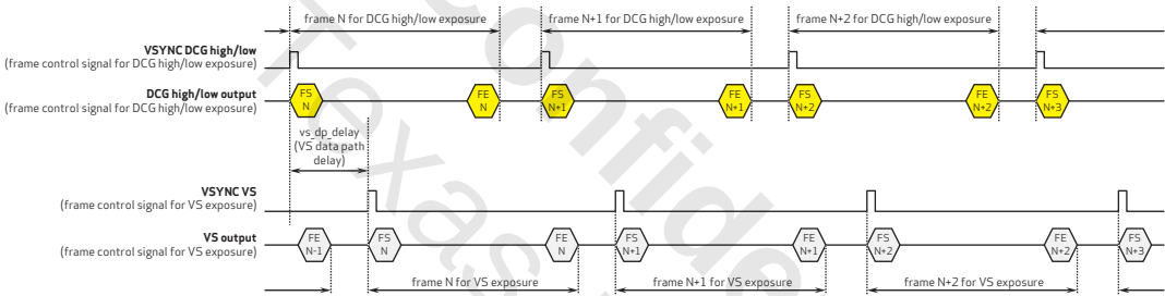
figure 5-27 sensor frame control signals diagram
