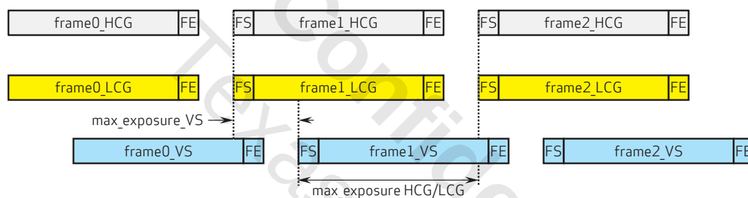
figure 5-5 staggered HDR with MIPI virtual channel diagram
