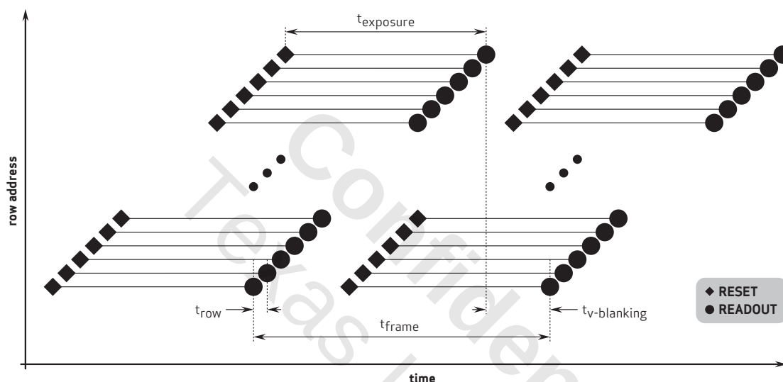
figure 3-8 row address versus time graph
