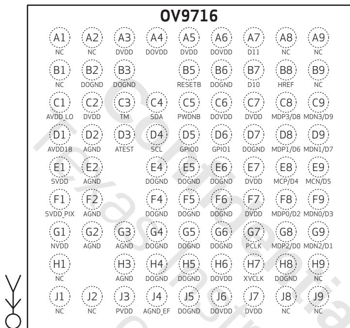
figure 1-3 pin diagram
