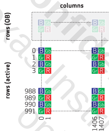
figure 3-2 pixel array region color filter layout
