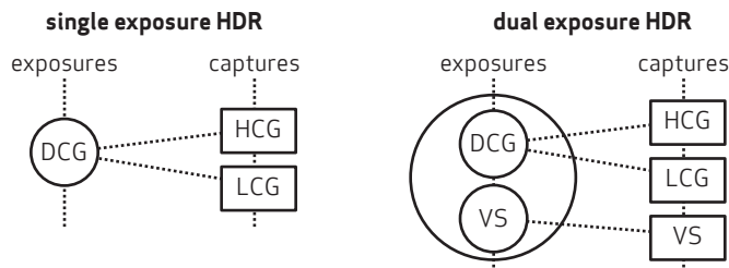
figure 3-3 exposures and captures diagram
