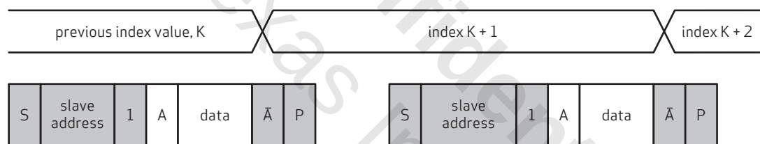
figure 6-4 SCCB single read from current location
