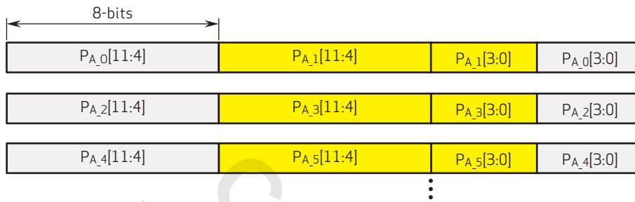
figure 5-17 12b compressed DCG single HDR diagram
