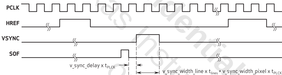
figure 5-20 DVP diagram
