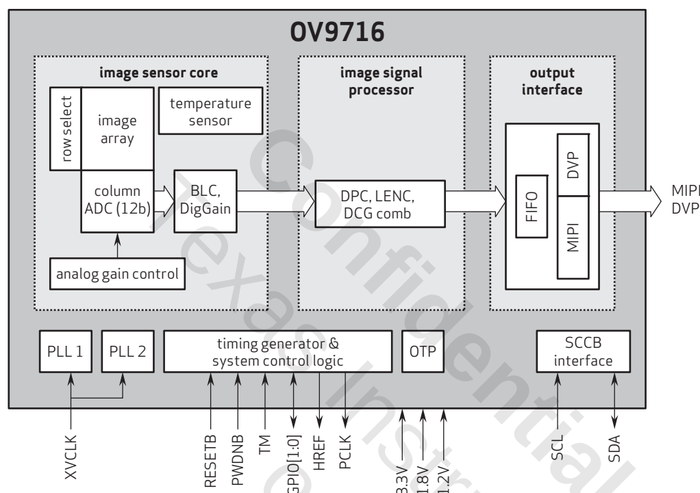
figure 2-1 OV9716 block diagram
