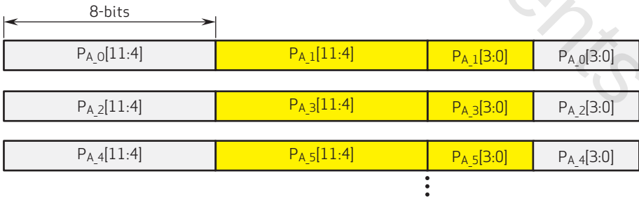
figure 5-11 12b linear mode diagram
