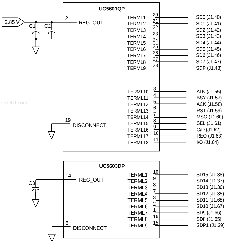
Figure 2.4 Regulated Termination
