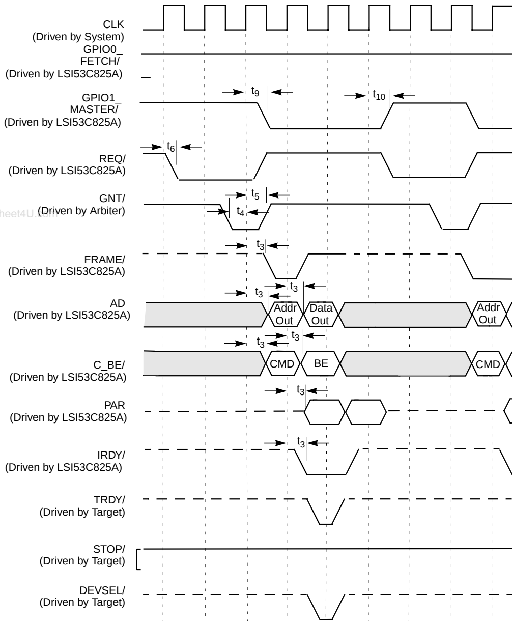
Figure 6.20 Burst Write
