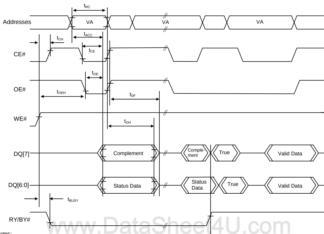
Figure 8. AC Waveforms for /DATA Polling During Embedded Algorithm Operations
