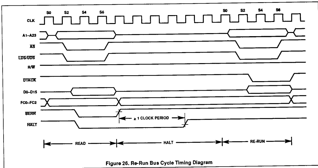
Figure 25. Bus Error Timing Diagram
