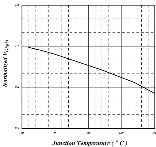
Fig 5. Gate Threshold Voltage v.s. Junction Temperature
