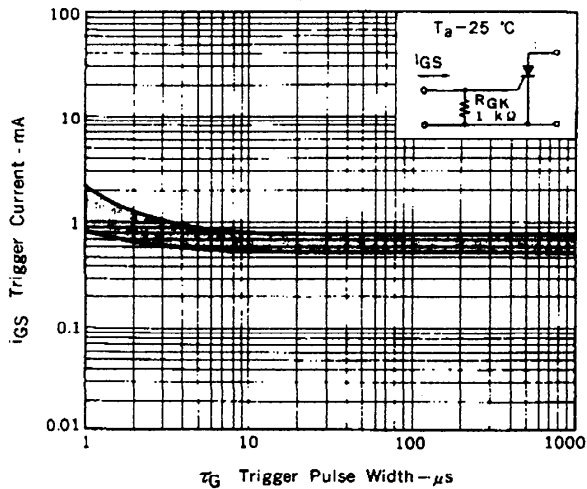
Fig. 7 I GS - τ G TYPICAL DISTRIBUTION
