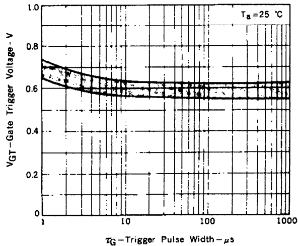
Fig. 8 V GT - τ G TYPICAL DISTRIBUTION
