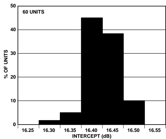
Figure 17. Intercept Histogram
