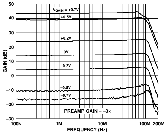
Figure 21. Frequency Response for Various Values of V_{\text{GAIN}} When the Preamplifier Gain is -3\times (See Figure 69 and Figure 57)
