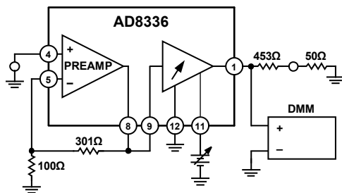
Figure 60. Offset Voltage
