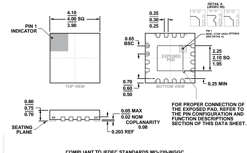
Figure 89. 16-Lead Lead Frame Chip Scale Package [LFCSP] 4 mm × 4 mm Body and 0.75 mm Package Height (CP-16-23) Dimensions shown in millimeters
