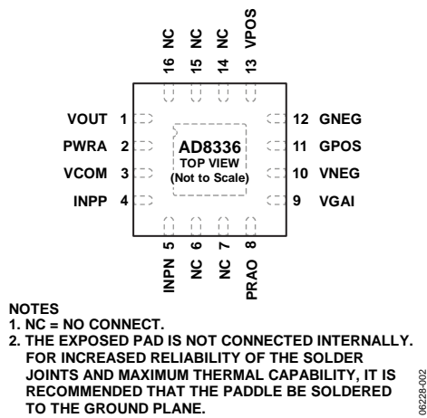
Figure 2. Pin Configuration
