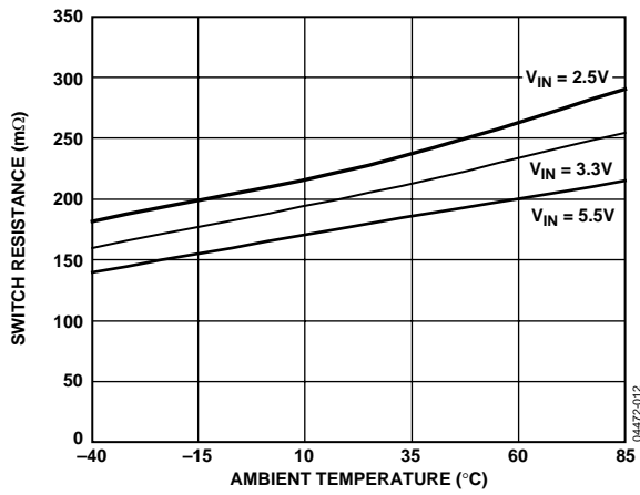
Figure 11. Switch Resistance vs. Ambient Temperature
