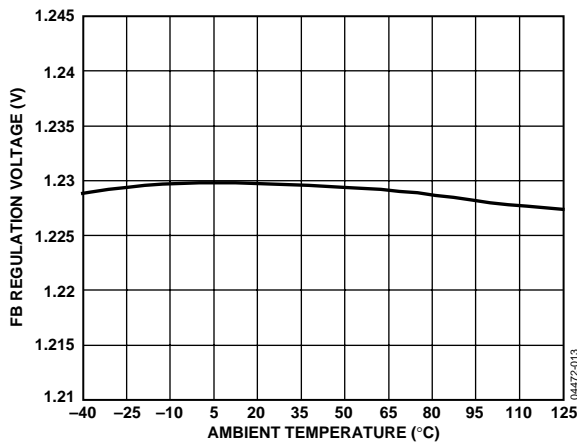
Figure 12. FB Regulation Voltage vs. Ambient Temperature
