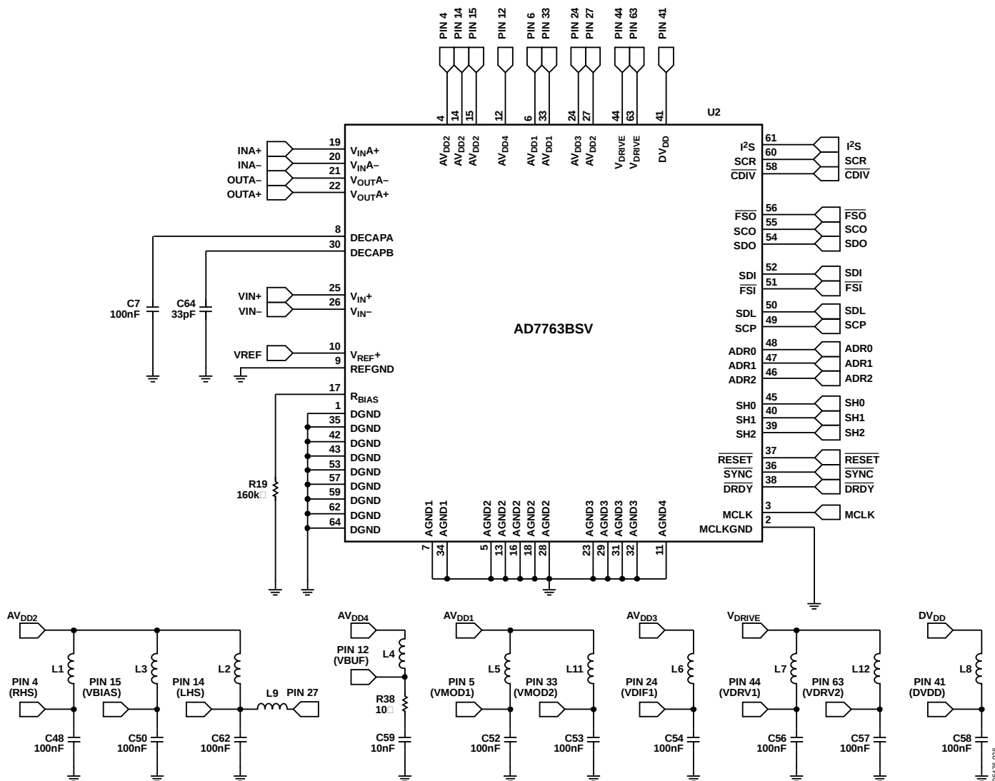
Figure 35. Simplified Connection Diagram
