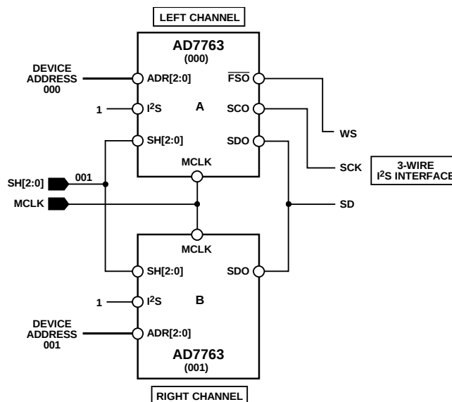
Figure 27. Two AD7763 Devices Operating Using the I 2 S Interface
