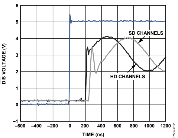
Figure 13. Enable Time
