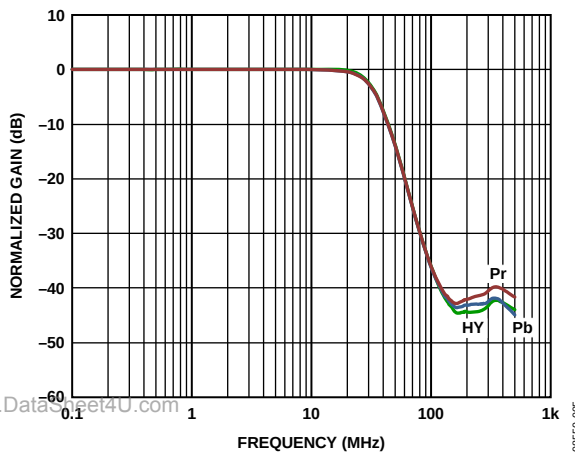
Figure 5. Frequency Response—ED Channels
