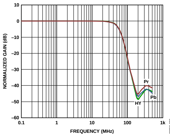
Figure 6. Frequency Response—HD Channels
