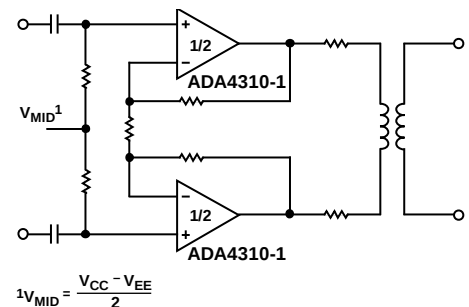
Figure 3. Typical PLC Driver Application
