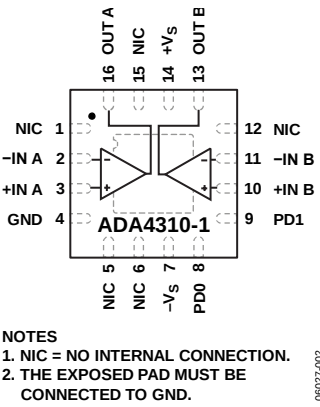
Figure 6. 16-Lead LFCSP Pin Configuration
