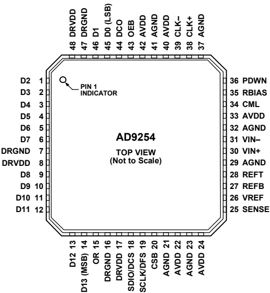
Figure 3. Pin Configuration
