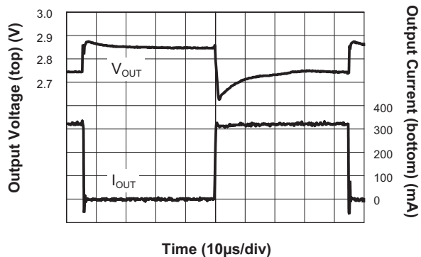
Load Transient Response 300mA ( V_{OUT} = 2.8\text{V} )
