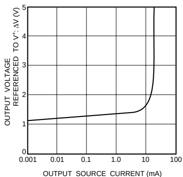
Fig. 7 Voltage difference during power supply output vs. output source current
