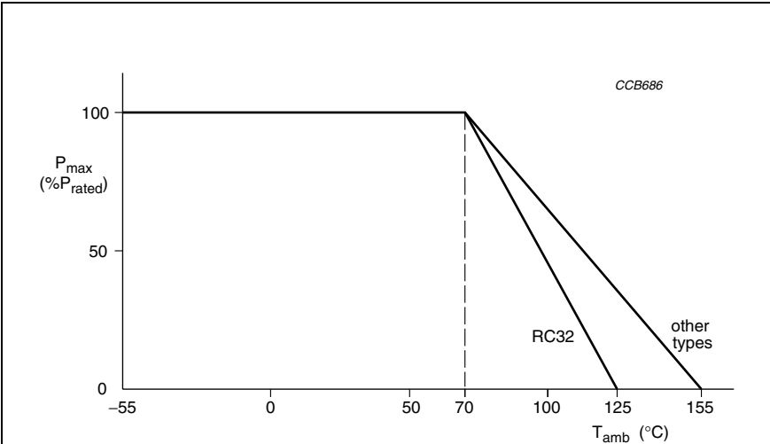
Fig.1 Maximum dissipation ( P_{max} ) in percentage of rated power as a function of the ambient temperature ( T_{amb} ).
