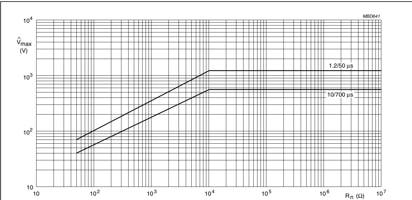
Fig.2 Maximum permissible peak pulse voltage without failing to 'open circuit' in accordance with DIN IEC 60040 (CO) 533 for type: RC02.
