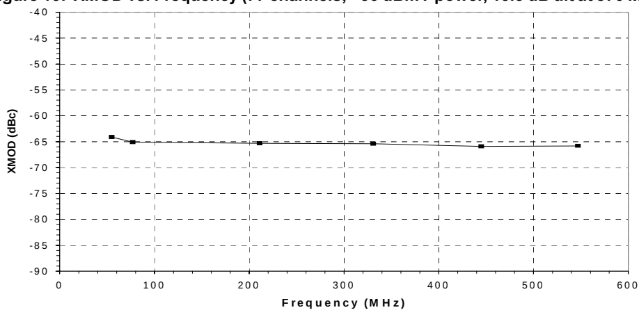
Figure 13: XMOD vs. Frequency (77 channels, +56 dBmV power, 13.5 dB tilt at 870 MHz)
