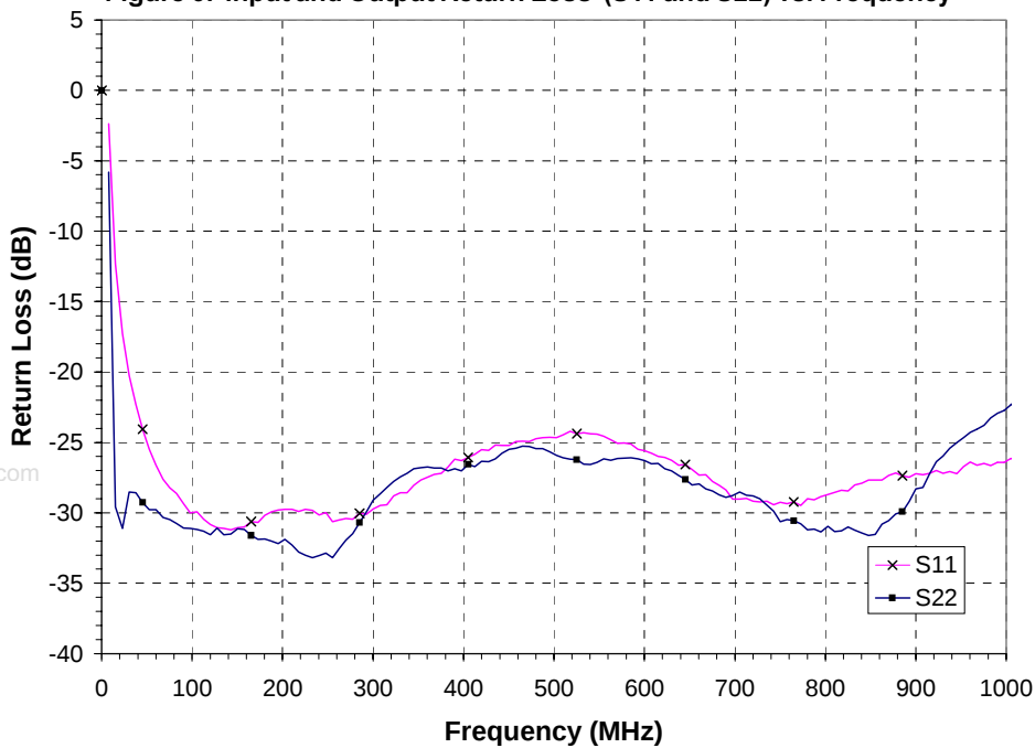
Figure 6: Input and Output Return Loss (S11 and S22) vs. Frequency
