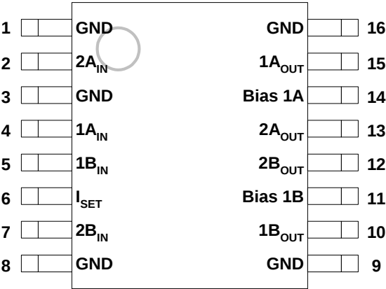
Figure 2: Pin Out
