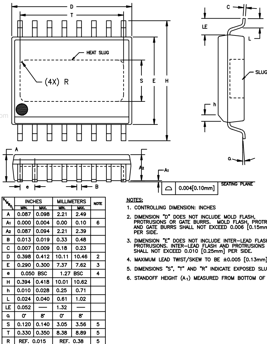
Figure 17: S7 Package Outline - 16 Pin Wide Body SOIC with Heat Slug
