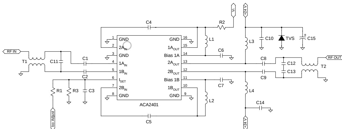
Figure 15: Evaluation Board Schematic
