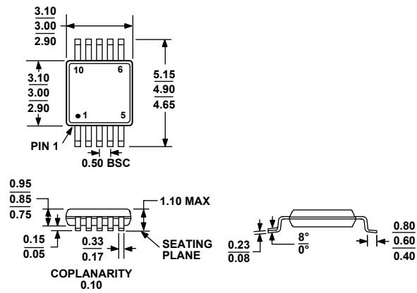
Figure 54. 10-Lead Mini Small Outline Package [MSOP] (RM-10) Dimensions shown in millimeters
