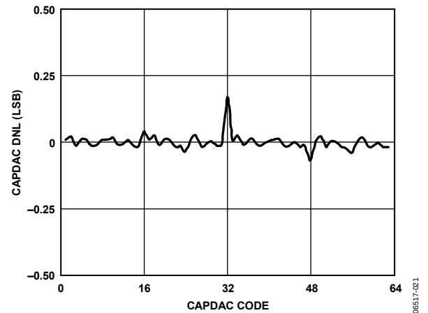
Figure 21. CAPDAC Differential Nonlinearity (DNL), V_{DD} = 3.3\text{ V}
