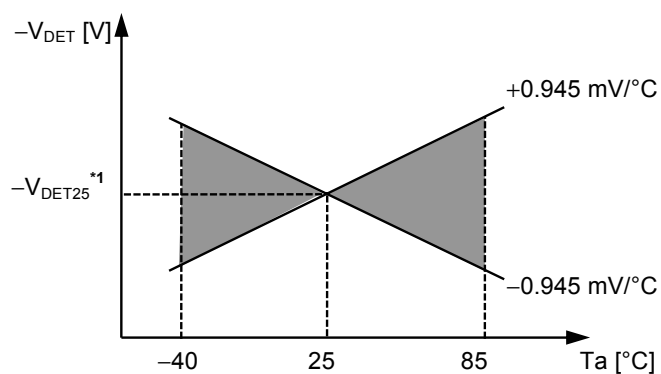
Figure 15 Temperature characteristics of detection voltage ( Example for -V_{DET} = 2.7 \text{ V} )
