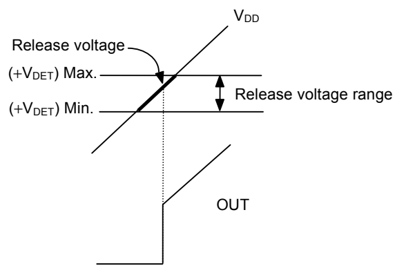
Figure 18 Release voltage (CMOS output products)
