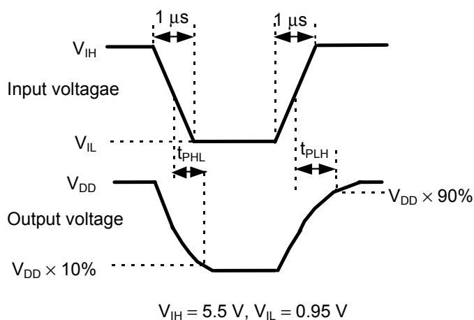
Figure 21 Measurement condition for response time
