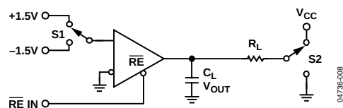
Figure 8. Receiver Enable/Disable
