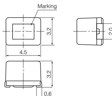
Type FB (4.5×3.2×3.2)
